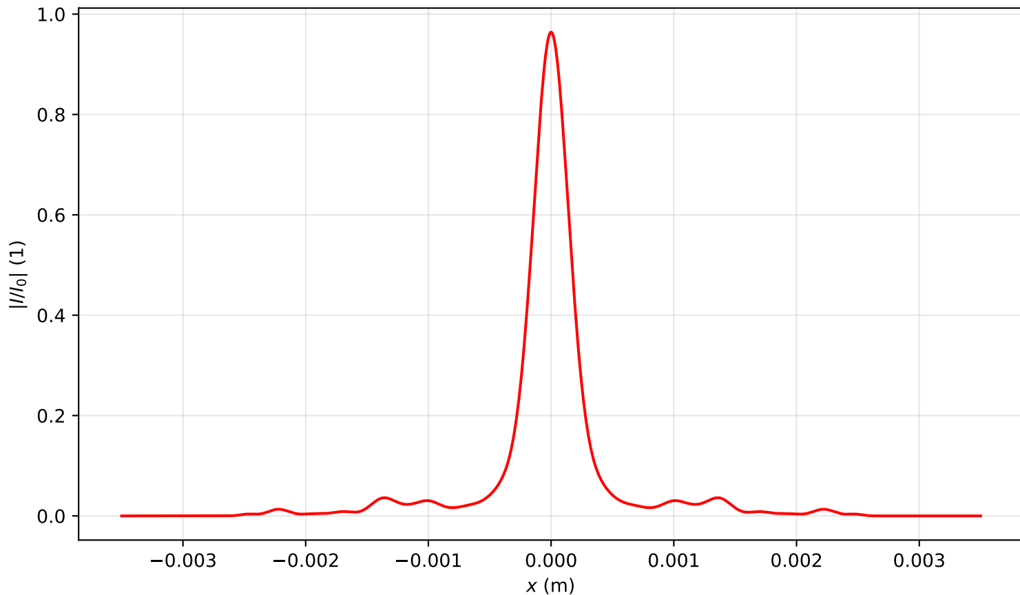
Intensity profile I(x, y = 0, z = 3.344)/I_0 , P_{in}=4.5P_{cr} , artificial time
